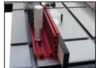
Router Table End View
