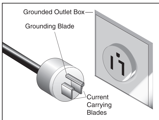
Figure 3. NEMA 5-30 plug and outlet.
